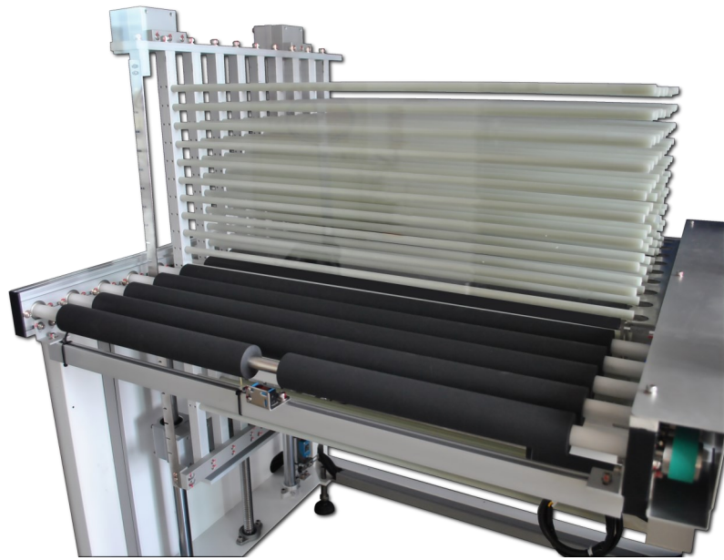
Buffer assembly
